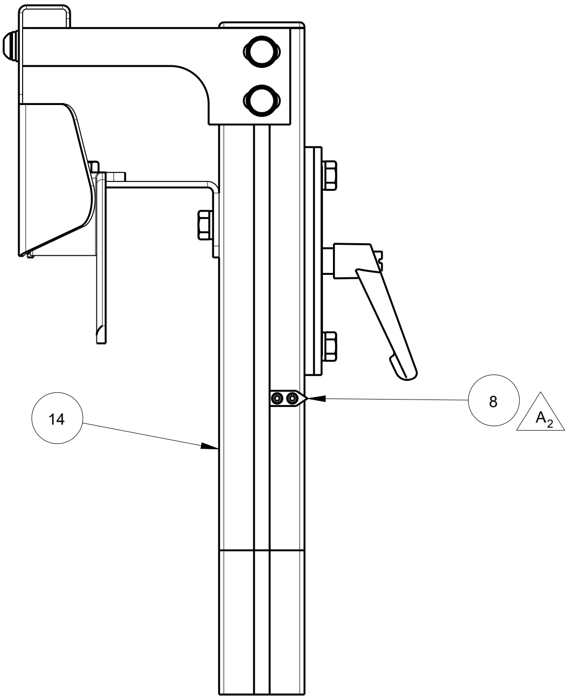
SCALE 1/2
